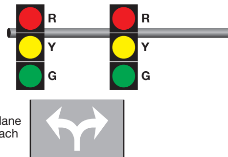
Figure 4F-15. Signal Indications for Approaches with Combined Left-Turn/Right-Turn Lane and No Through Movement (Sheet 3 of 3)
