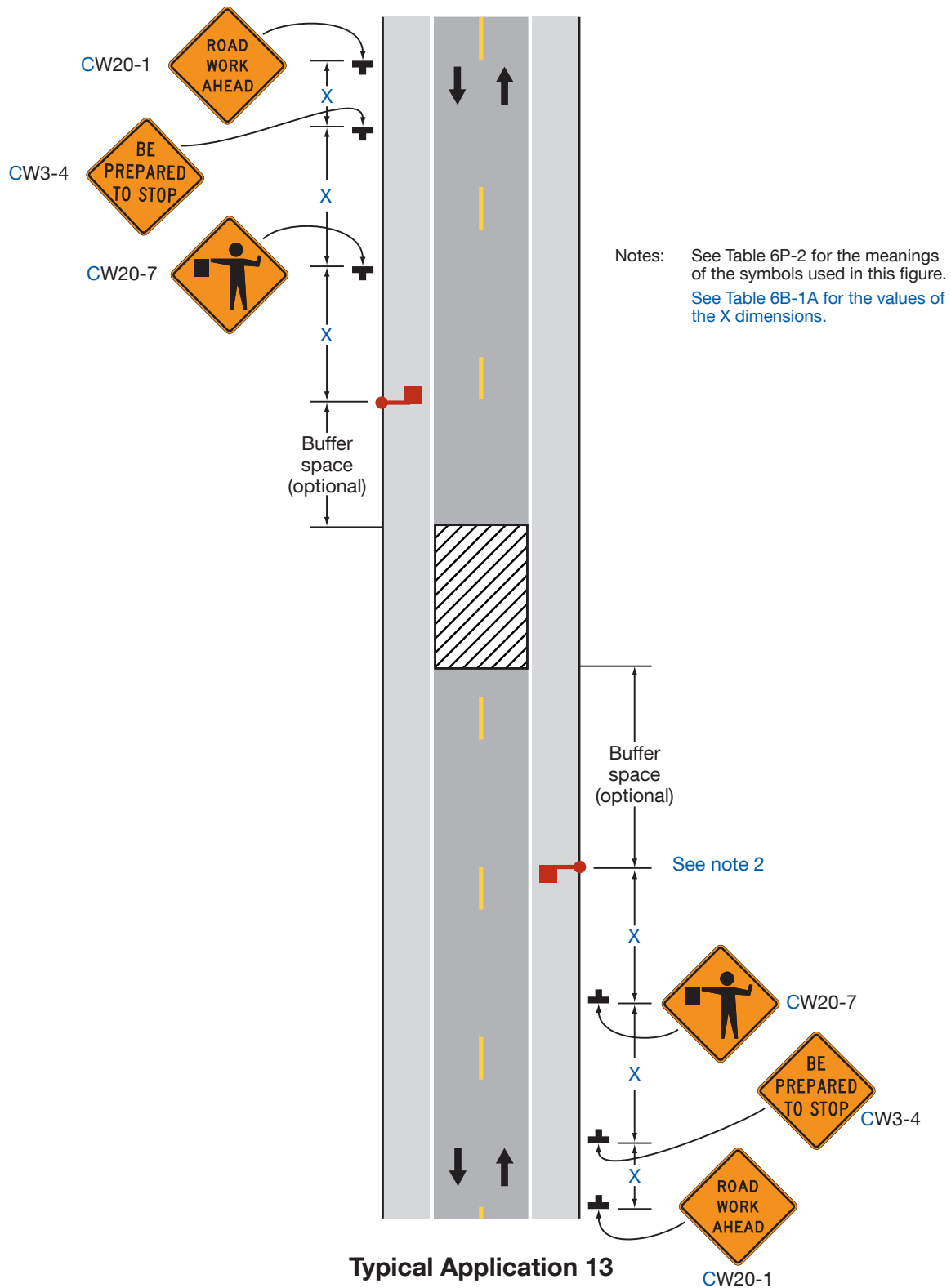
Figure 6P-13. Temporary Road Closure (TA-13)
