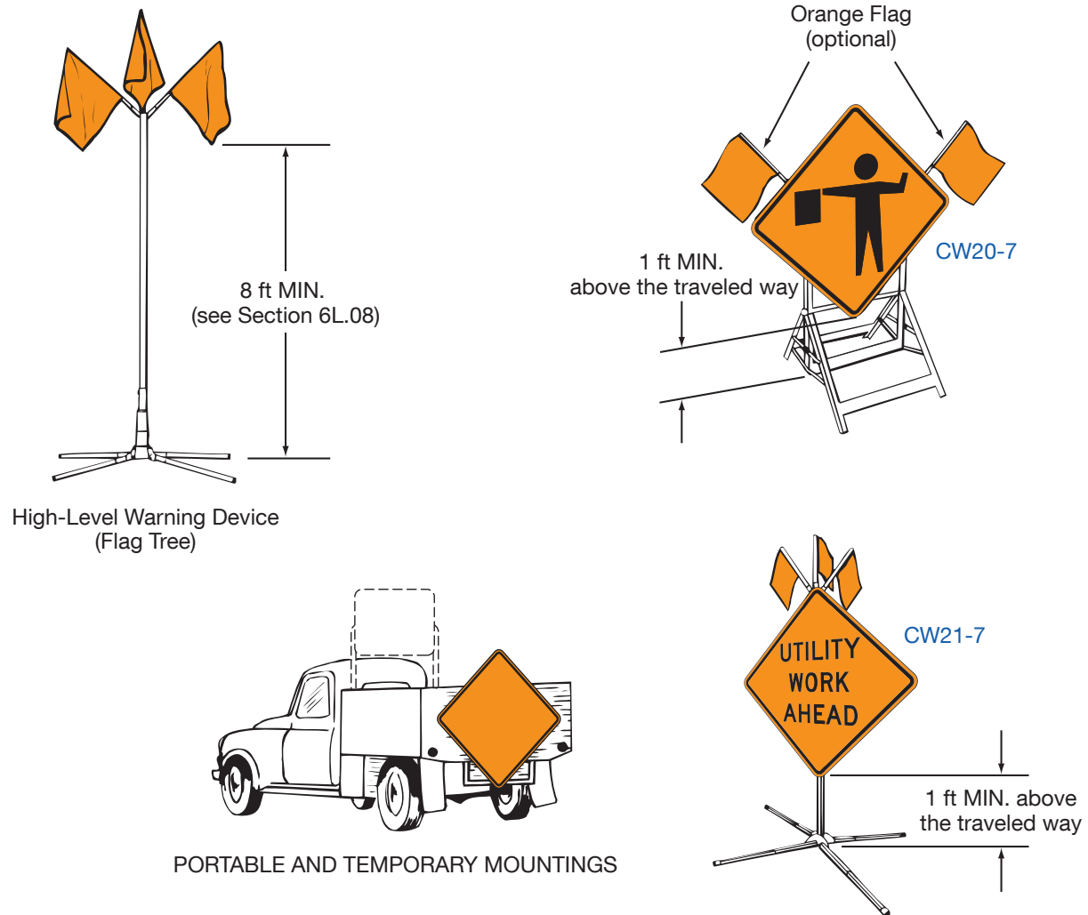
Figure 6F-2. Methods of Mounting Signs Other Than on Posts
