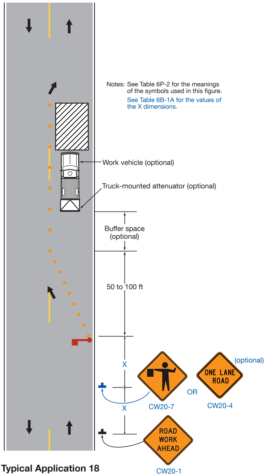
Figure 6P-18. Lane Closure on a Minor Street (TA-18)
