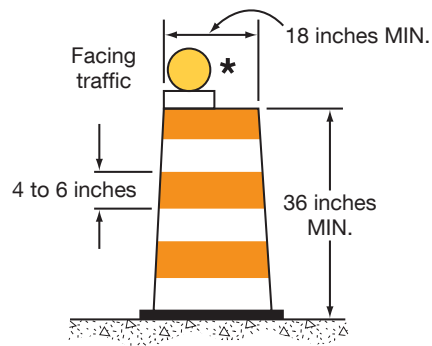
Figure 6K-1. Examples of Channelizing Devices (Sheet 1 of 2)
