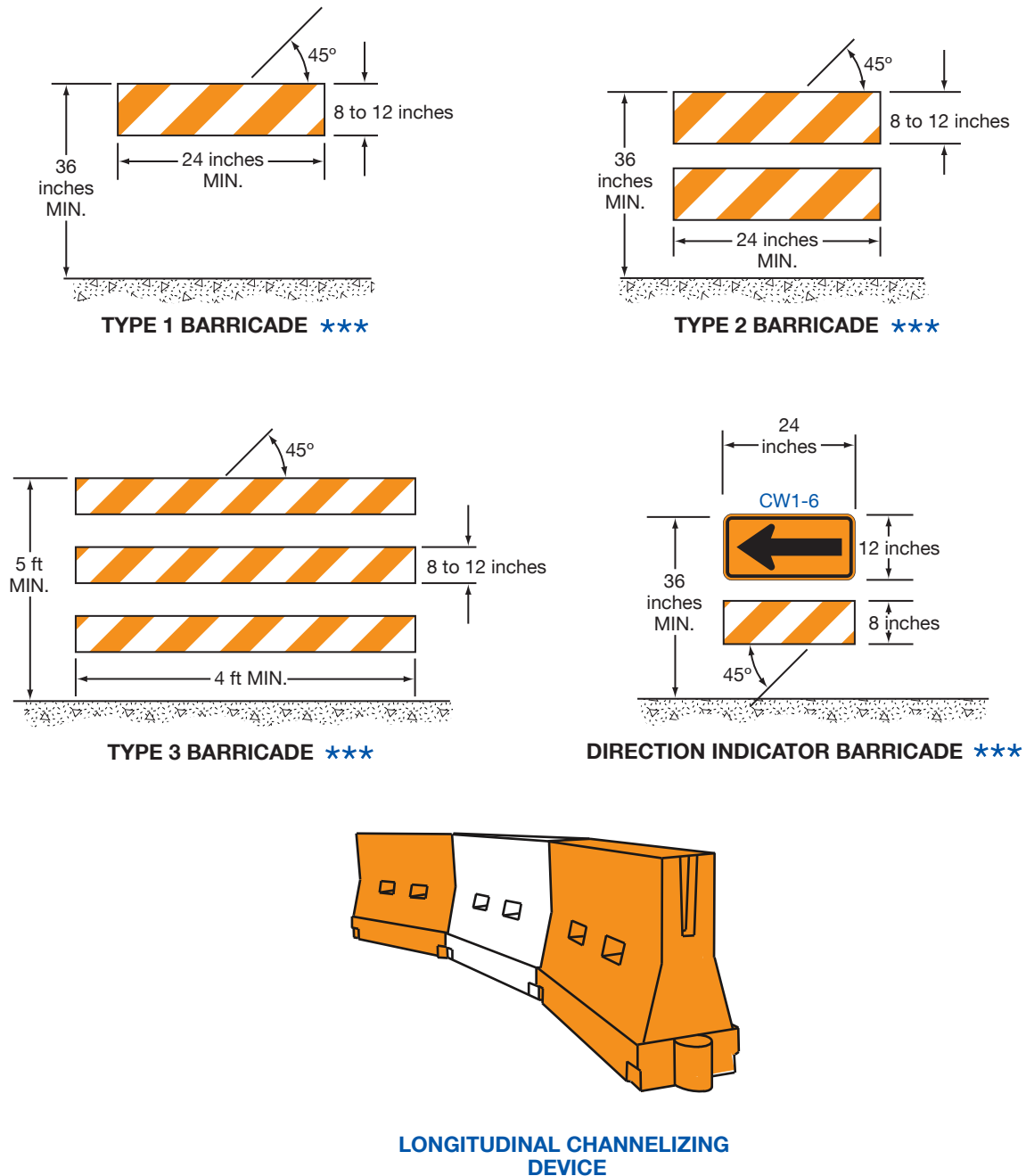
Figure 6K-1. Examples of Channelizing Devices (Sheet 2 of 2)
