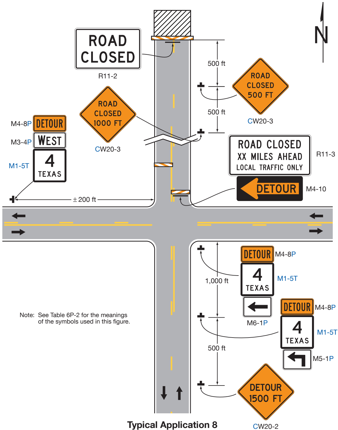
Figure 6P-8. Road Closure with an Off-Site Detour (TA-8)
