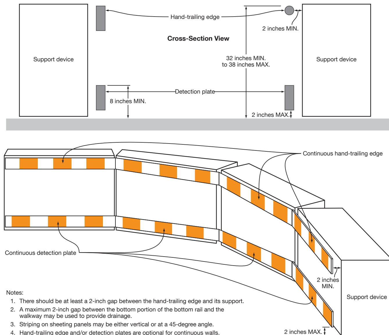
Figure 6K-2. Pedestrian Channelizing Device
