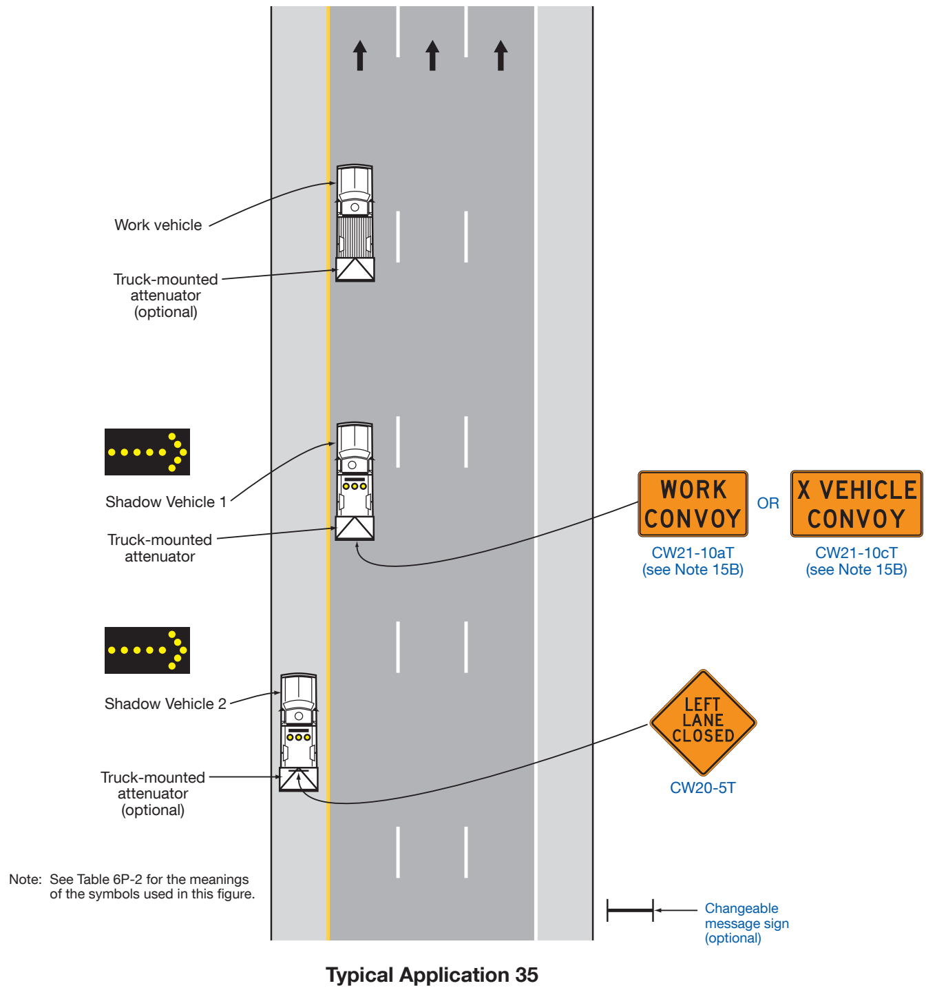
Figure 6P-35. Mobile Operation on a Multi-Lane Road (TA-35)
