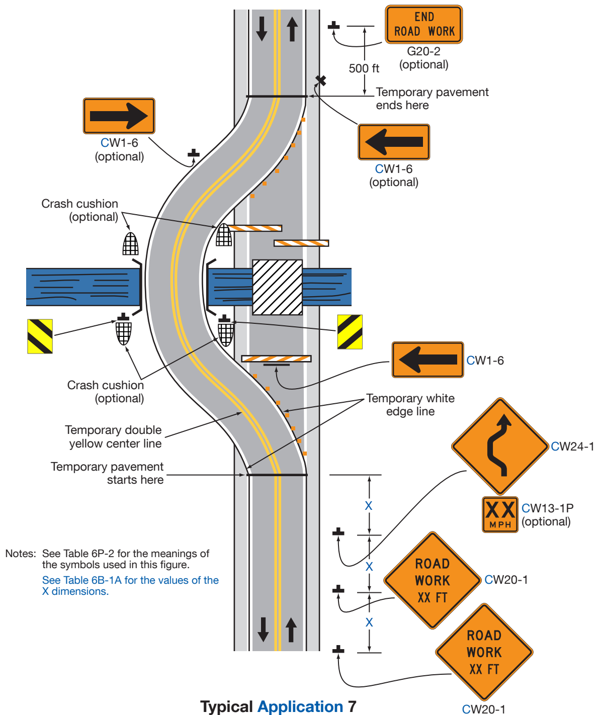
Figure 6P-7. Road Closure with a Diversion (TA-7)
