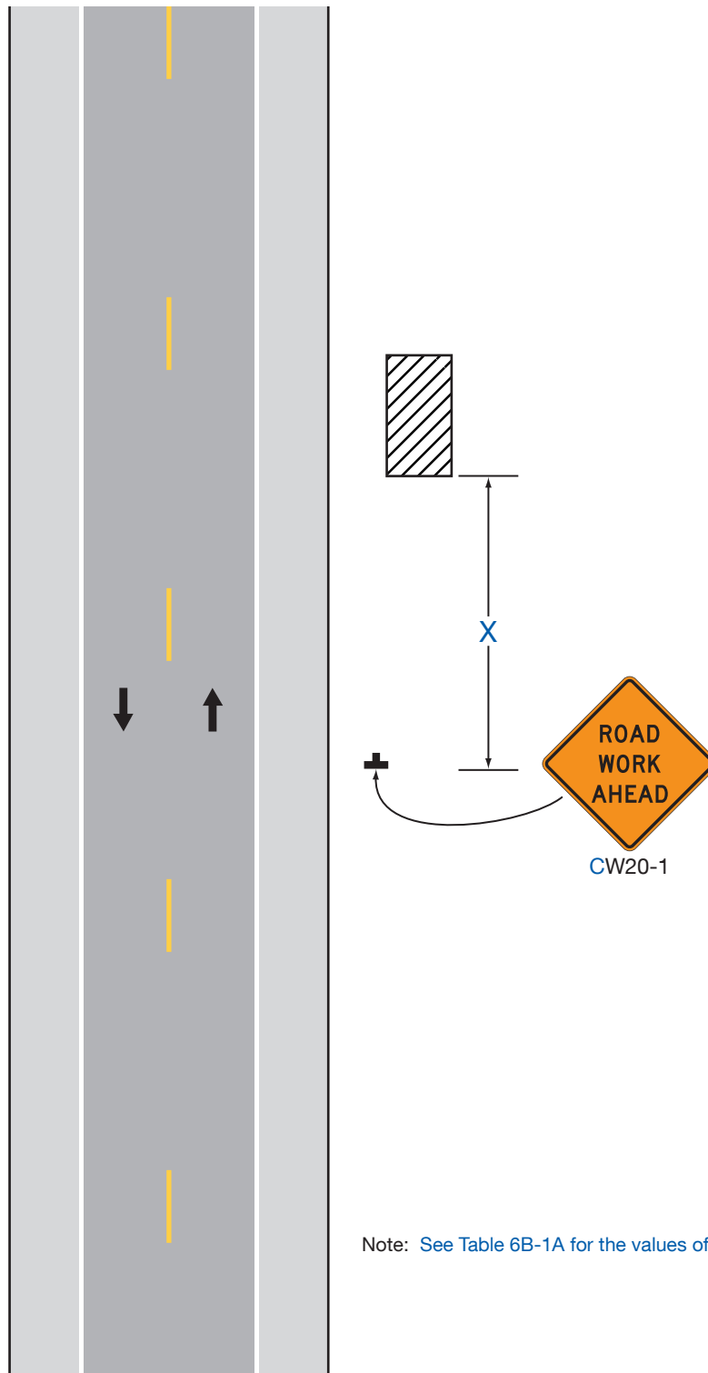
Figure 6P-1. Work Beyond the Shoulder (TA-1)
