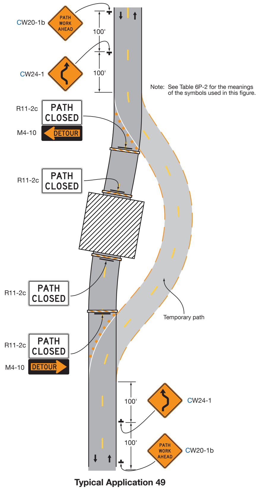
Figure 6P-49. Shared-Use Path Closure with a Diversion (TA-49)
