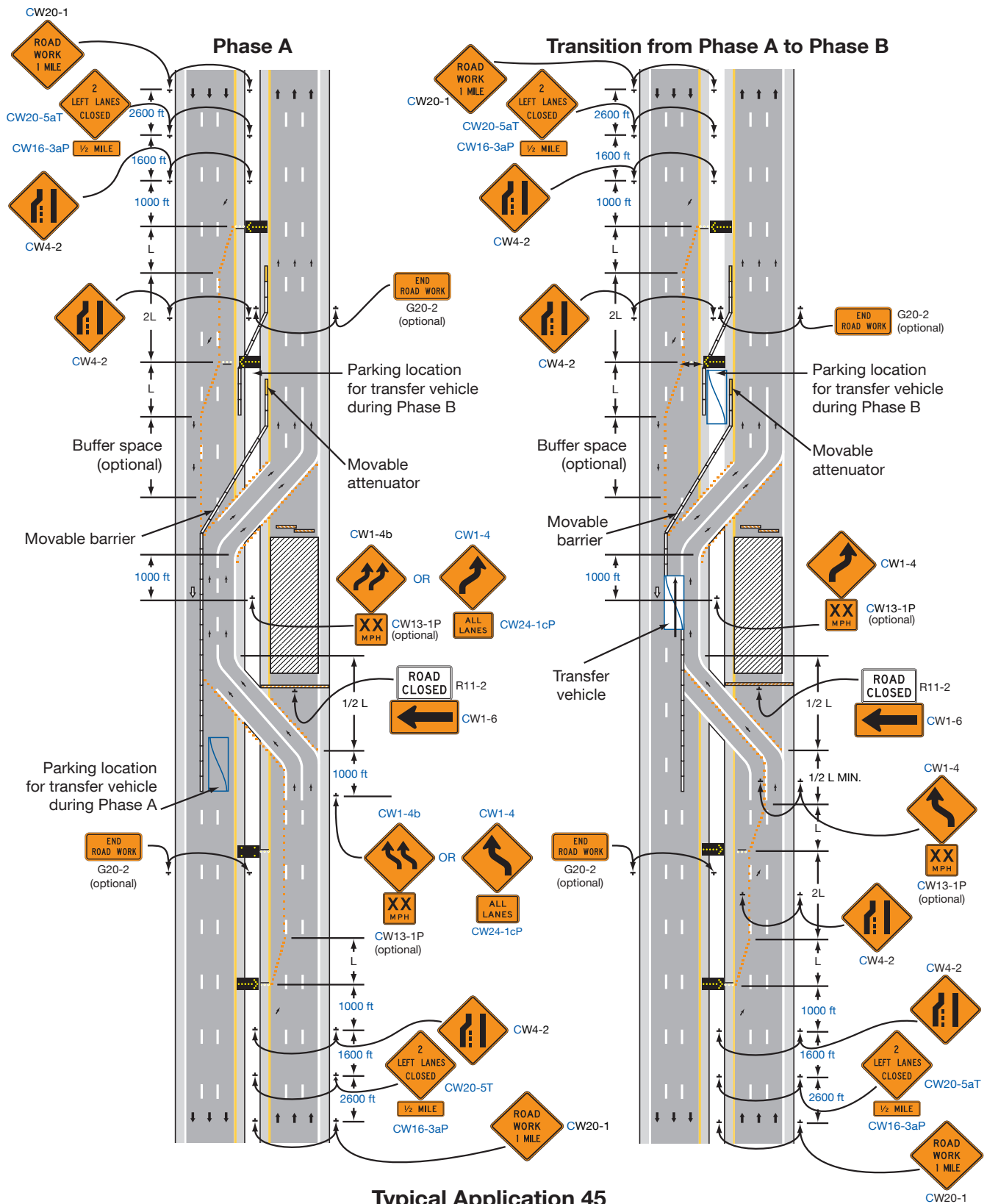
Figure 6P-45. Temporary Reversible Lane Using Movable Barriers (TA-45)
