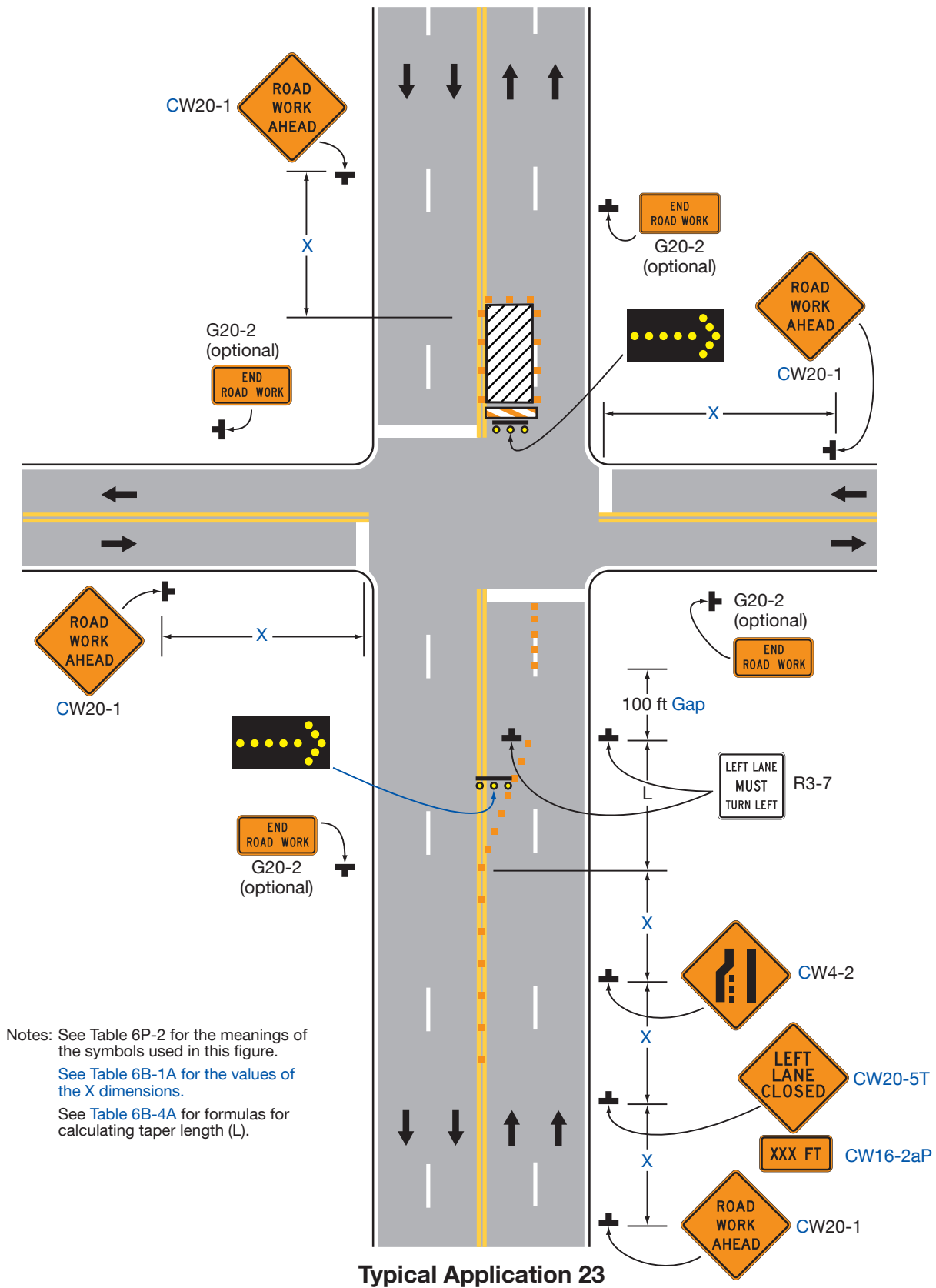
Figure 6P-23. Left-Hand Lane Closure on the Far Side of an Intersection (TA-23)
