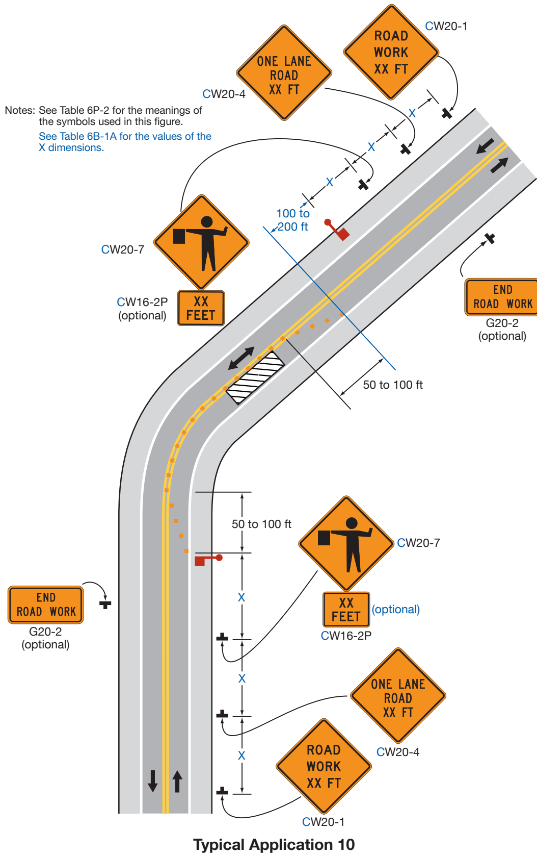
Figure 6P-10. Lane Closure on Two-Lane Road Using Flaggers (TA-10)
