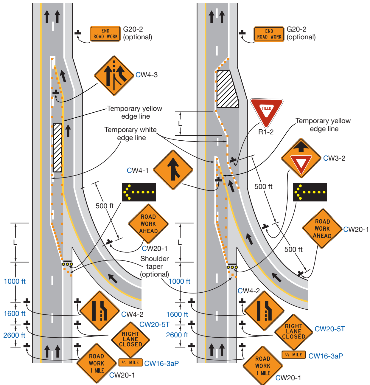
Figure 6P-44. Work in the Vicinity of an Entrance Ramp (TA-44)
