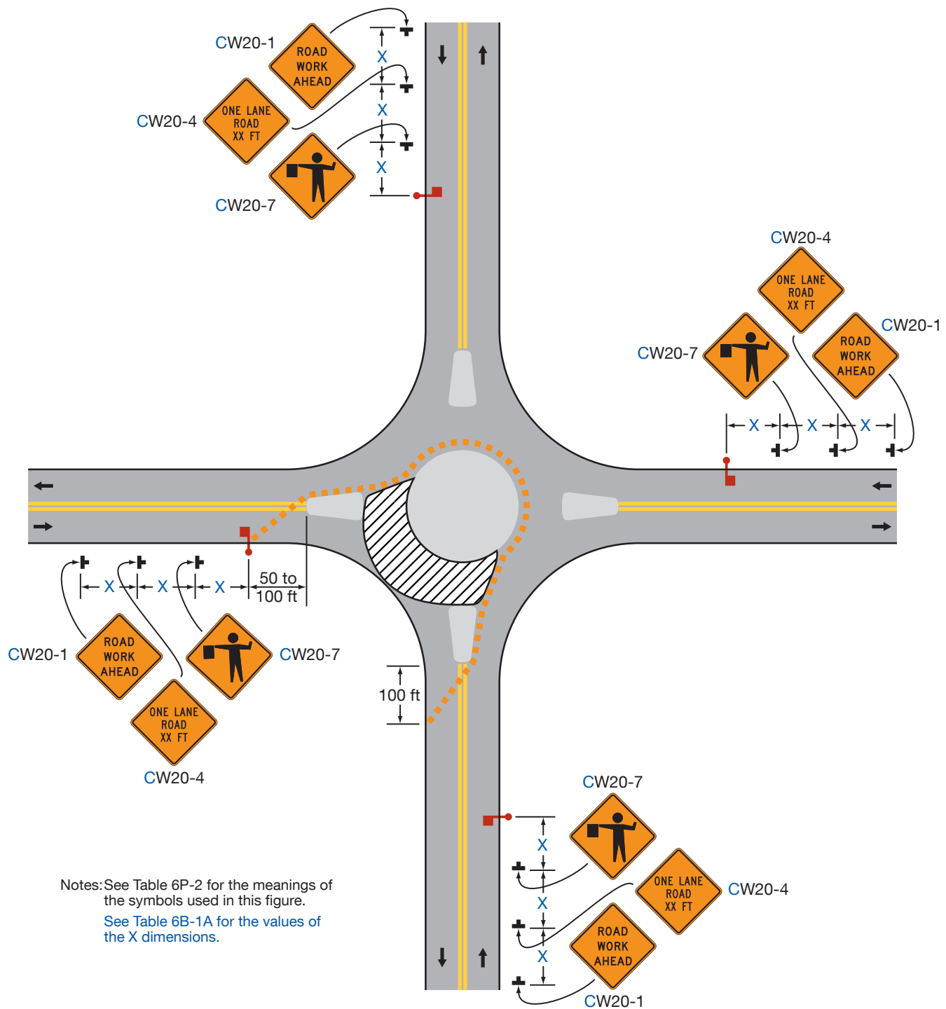
Figure 6P-52. Short-Term or Short-Duration Work in a Circular Intersection (TA-52)
