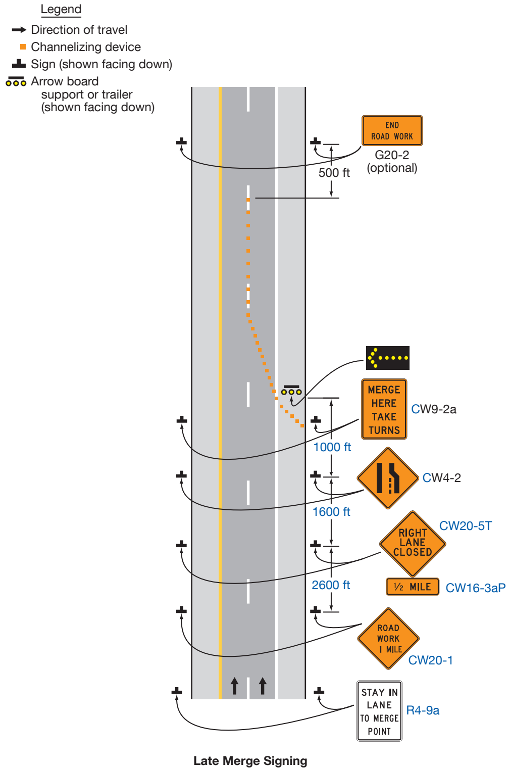
Figure 6N-1. Late Merge
