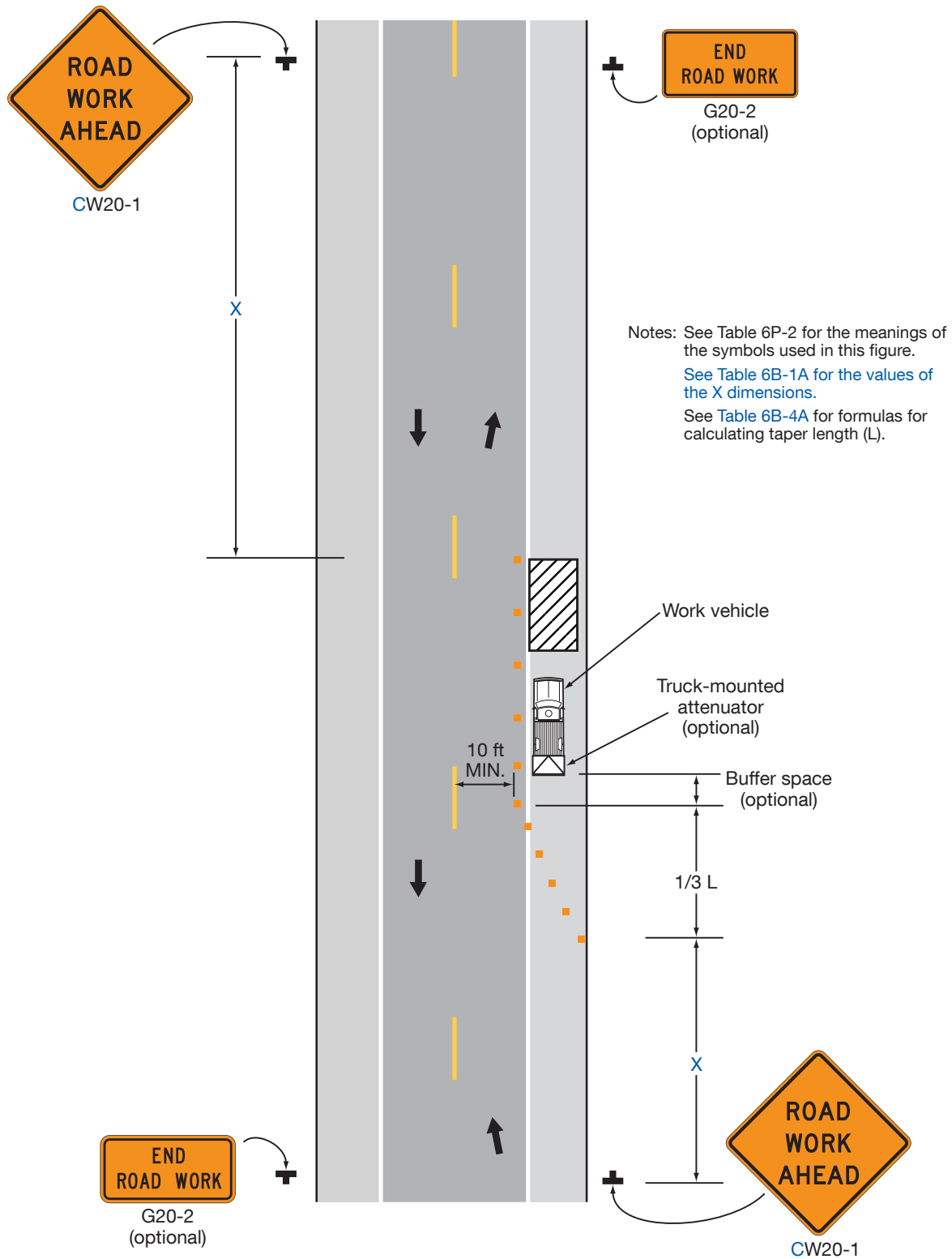
Figure 6P-6. Shoulder Work with Minor Encroachment (TA-6)
