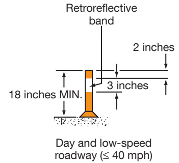
Figure 6K-1. Examples of Channelizing Devices (Sheet 1 of 2)
