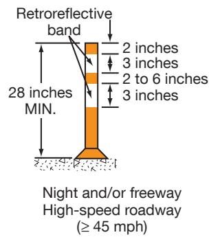
Figure 6K-1. Examples of Channelizing Devices (Sheet 1 of 2)
