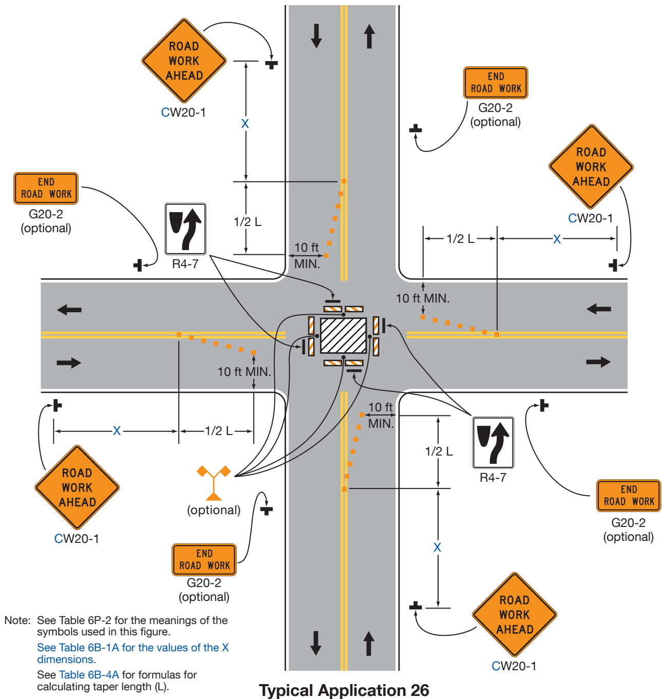
Figure 6P-26. Closure in the Center of an Intersection (TA-26)
