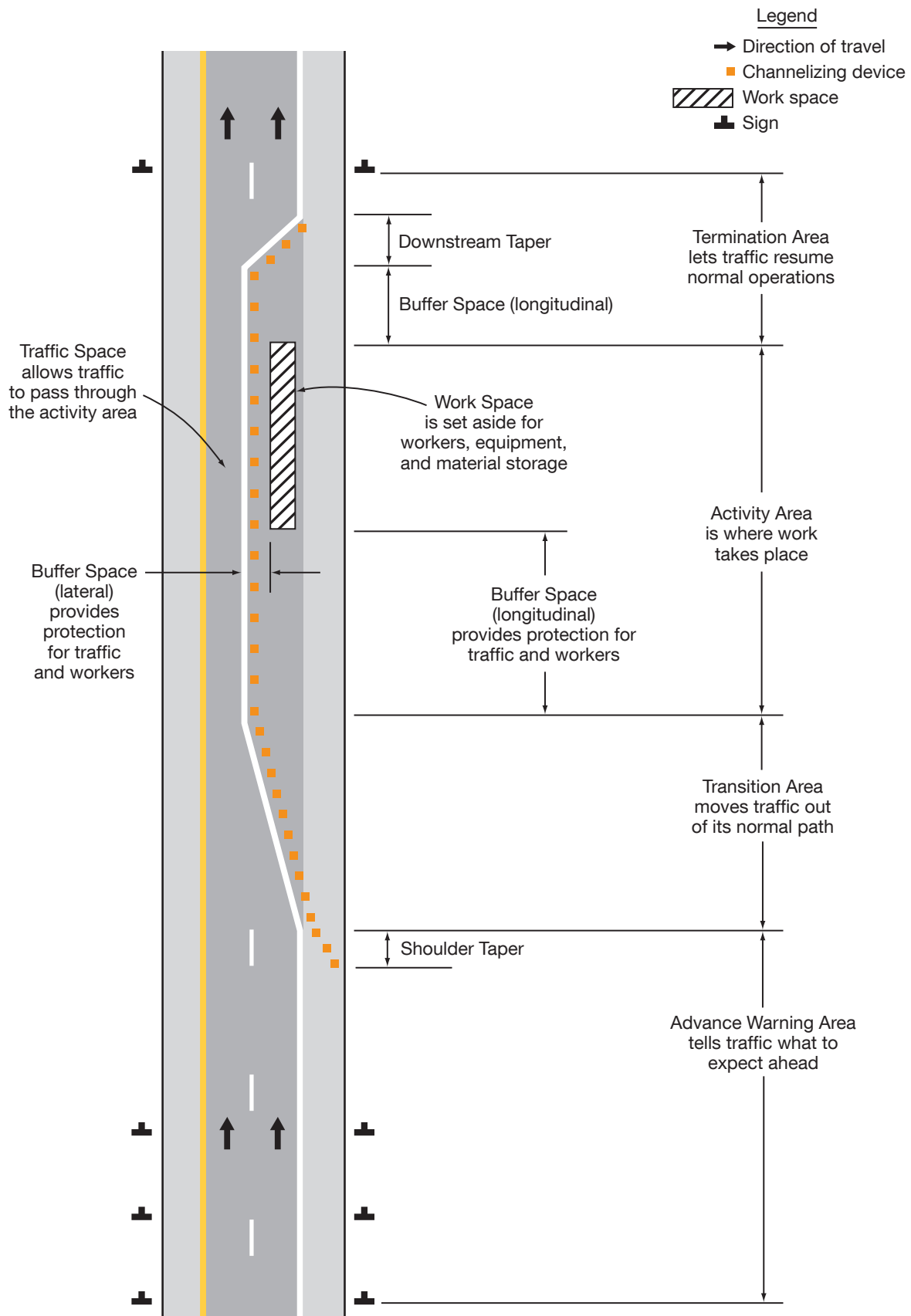
Figure 6B-1. Component Parts of Temporary Traffic Control Zone
