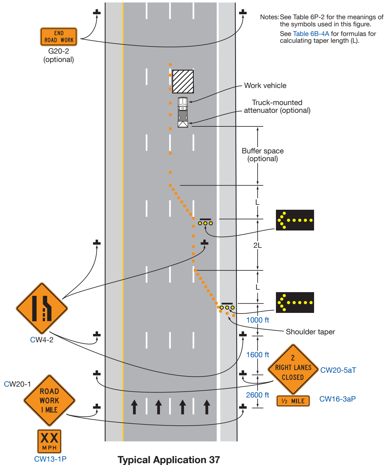
Figure 6P-37. Double Lane Closure on a Freeway (TA-37)
