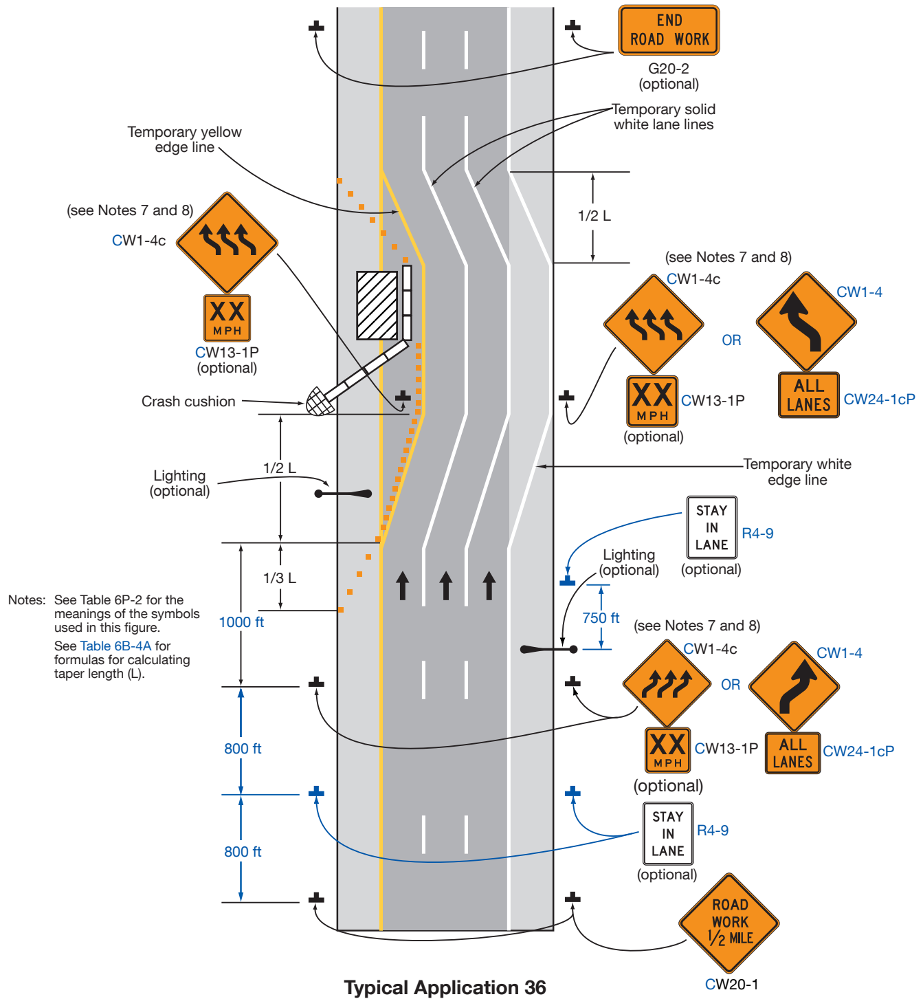
Figure 6P-36. Lane Shift on a Freeway (TA-36)
