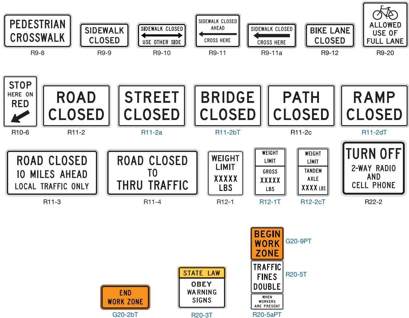
Figure 6G-1. Regulatory Signs and Plaques in Temporary Traffic Control Zones (Sheet 2 of 2)
