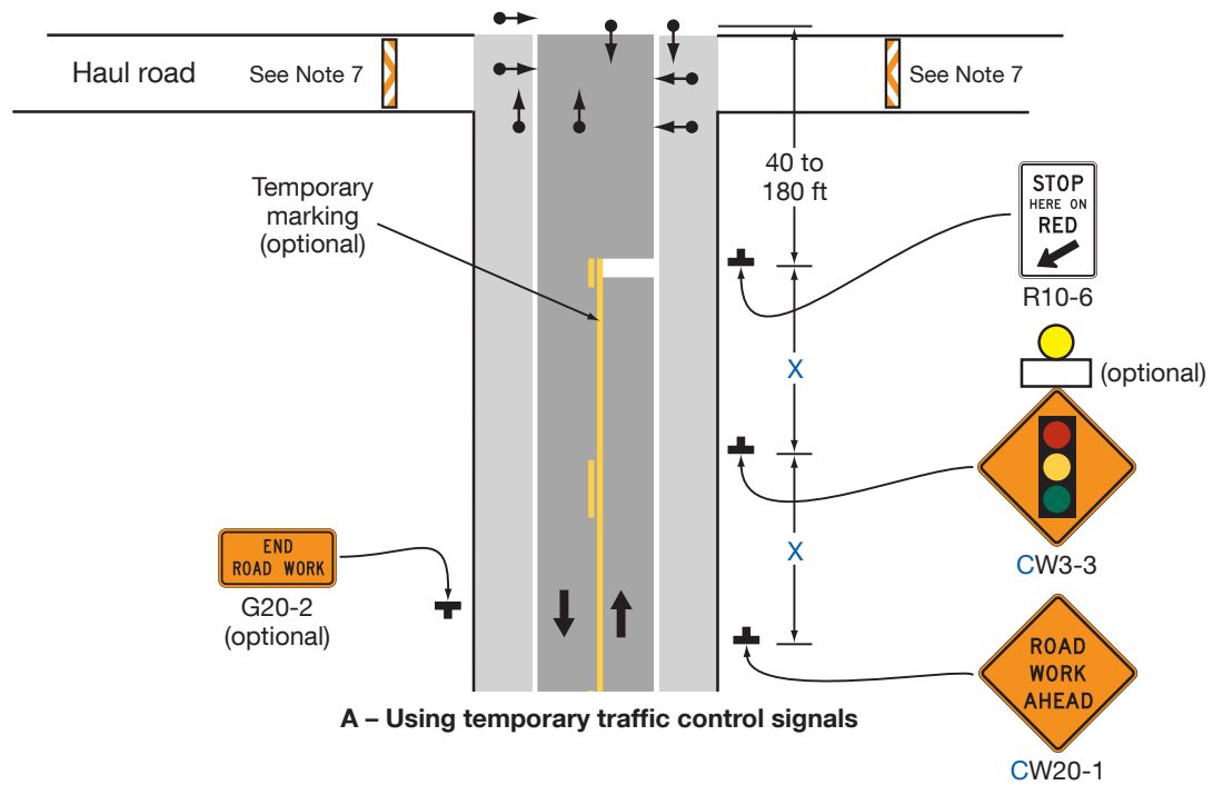
Figure 6P-14. Haul Road Crossing (TA-14)
