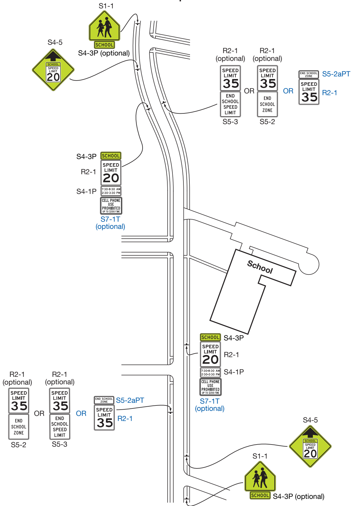
Figure 7B-4. Example of Signing for a Cell Phone Use Prohibited with a School Speed Limit
