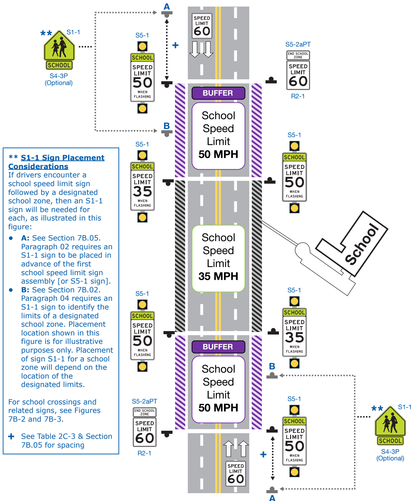
Figure 7B-4A. (TX) Example of a Buffer School Speed Zone
